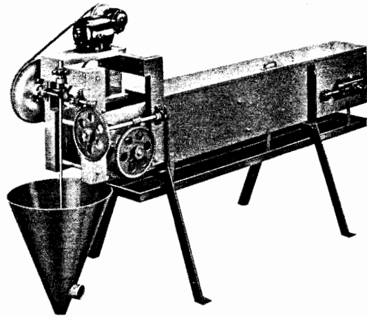
BELT TYPE ZINC FEEDER
