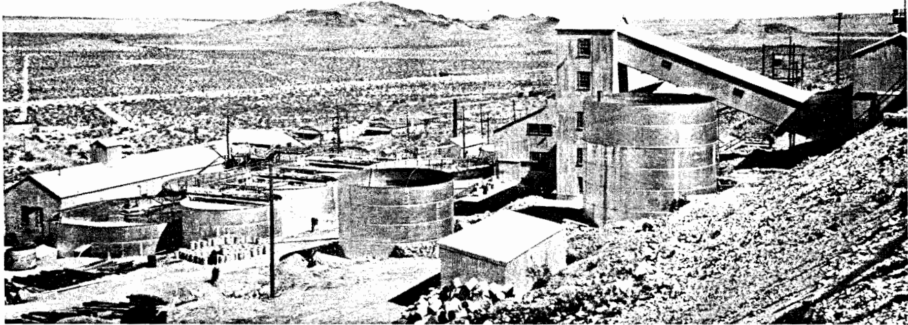
Golden Queen Mill, Mojave, California. This thoroughly modern all cyanidation plant has a rated capacity of from 350 to 400 tons of ore per day, and the equipment includes a Merrill-Crowe Simultaneous Clarification-Precipitation Unit with a daily capacity of 1000 tons of solution.
